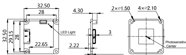
Undeclared tolerance:±0.1
