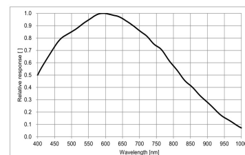
MER2-041-436U3M
